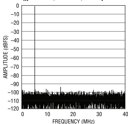
LTC2266-12: 8k Point FFT, f_{IN} = 5\text{MHz} , -1\text{dBFS} , 80Msps
