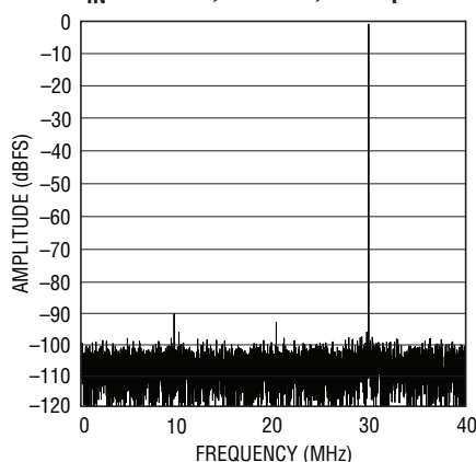
LTC2266-12: 8k Point FFT, f_{IN} = 30\text{MHz} , -1\text{dBFS} , 80Msps
