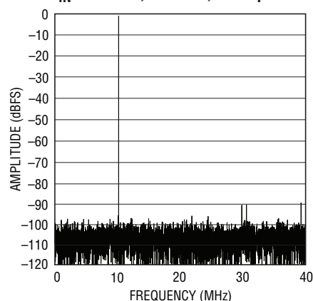
LTC2266-12: 8k Point FFT, f_{IN} = 70\text{MHz} , -1\text{dBFS} , 80Msps
