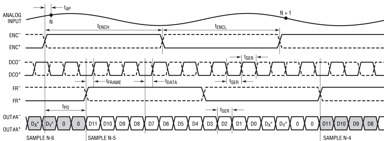
1-Lane Output Mode, 16-Bit Serialization
