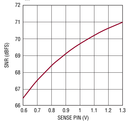
LTC2268-12: SNR vs SENSE, f_{IN} = 5\text{MHz} , -1dBFS
