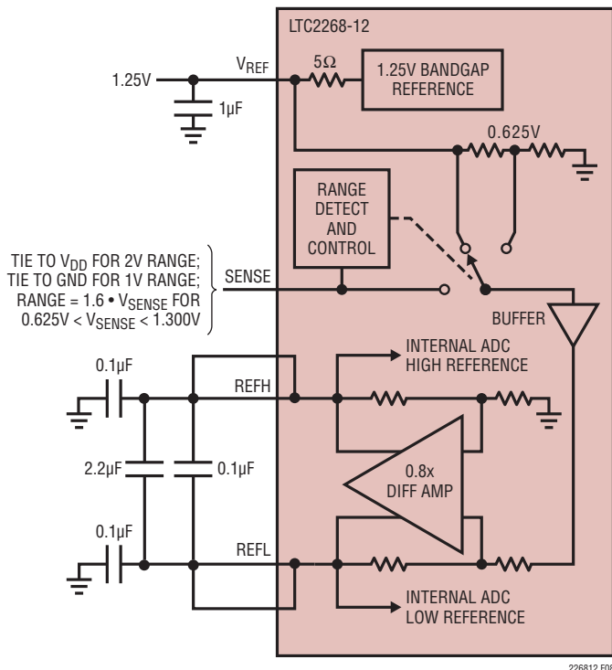
Figure 8. Reference Circuit
